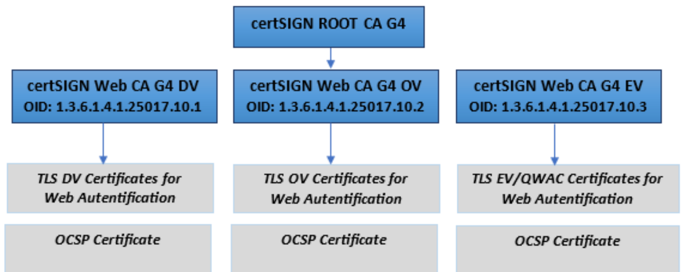
Figure 1: certSIGN ROOT CA G4 certification domain structure
